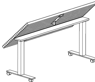
Nesting - Fixed kid's height (24" AFF) / castor base
